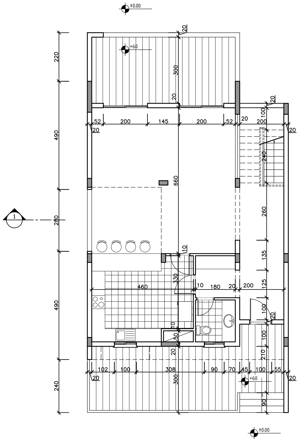
GROUND FLOOR PLAN Sc. 1/100
