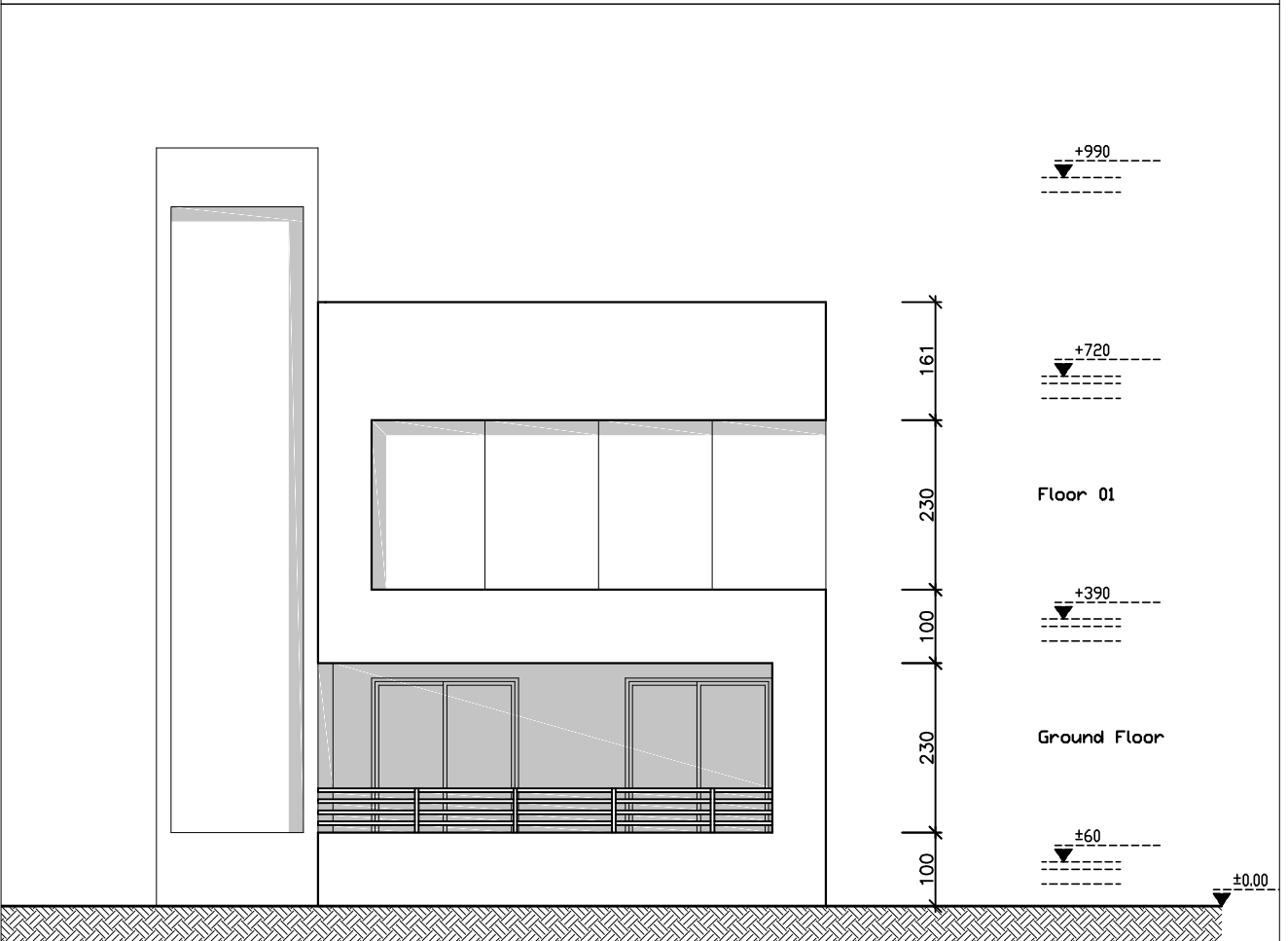
SECTION 1 Sc. 1/100
