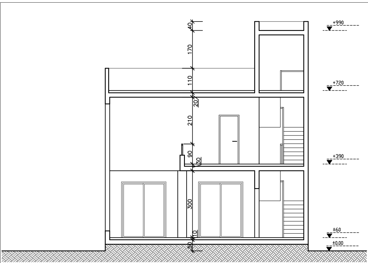
SECTION 1 Sc. 1/100
