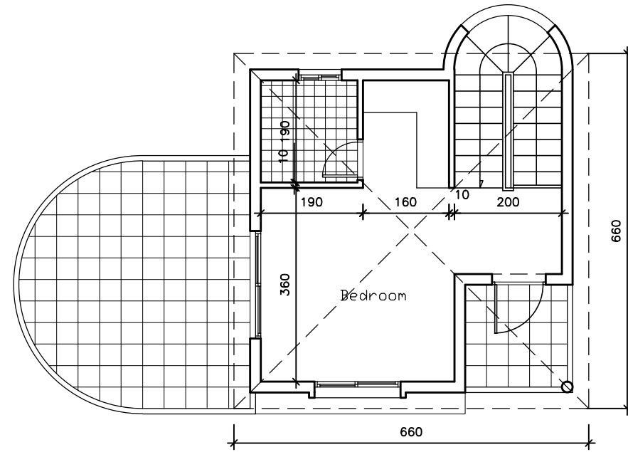
1st Floor Plan Sc. 1/100
