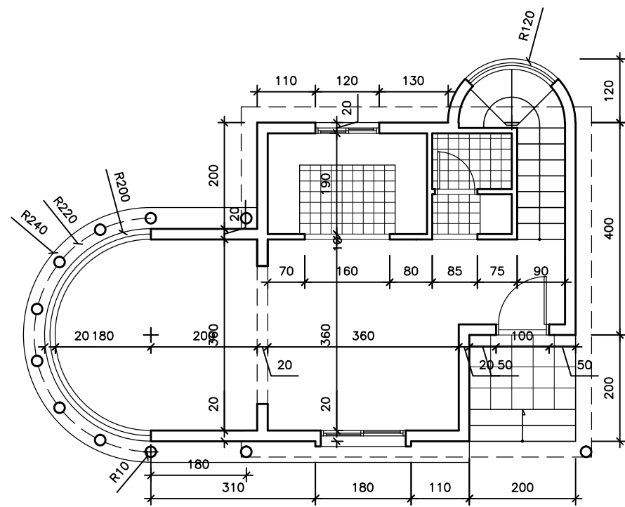
Ground Floor Plan Sc. 1/100
